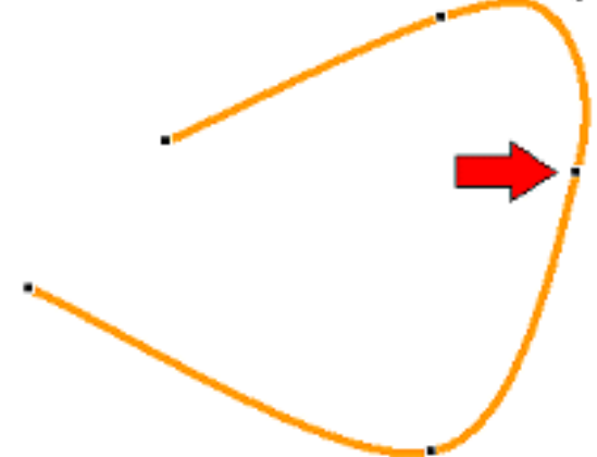
C_0 & C_1 & C_2 continuity
