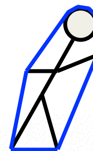
Convex Hull
